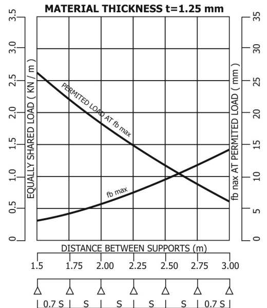
CABLE TRAY H:110 LOADING DIAGRAM
